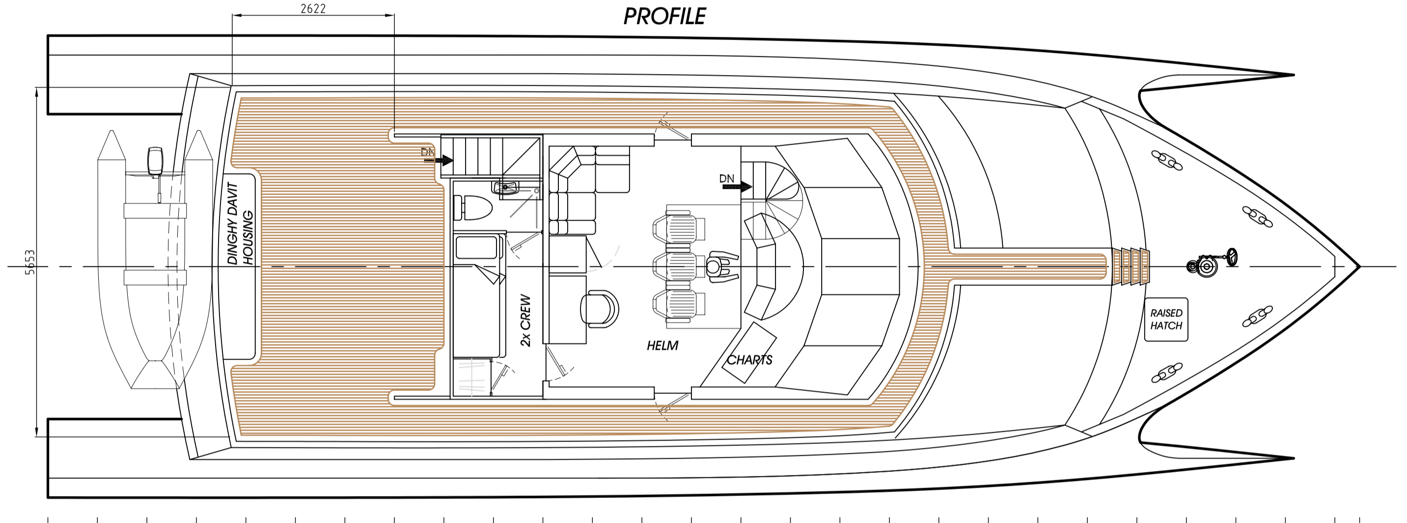
UPPERDECK PLAN
