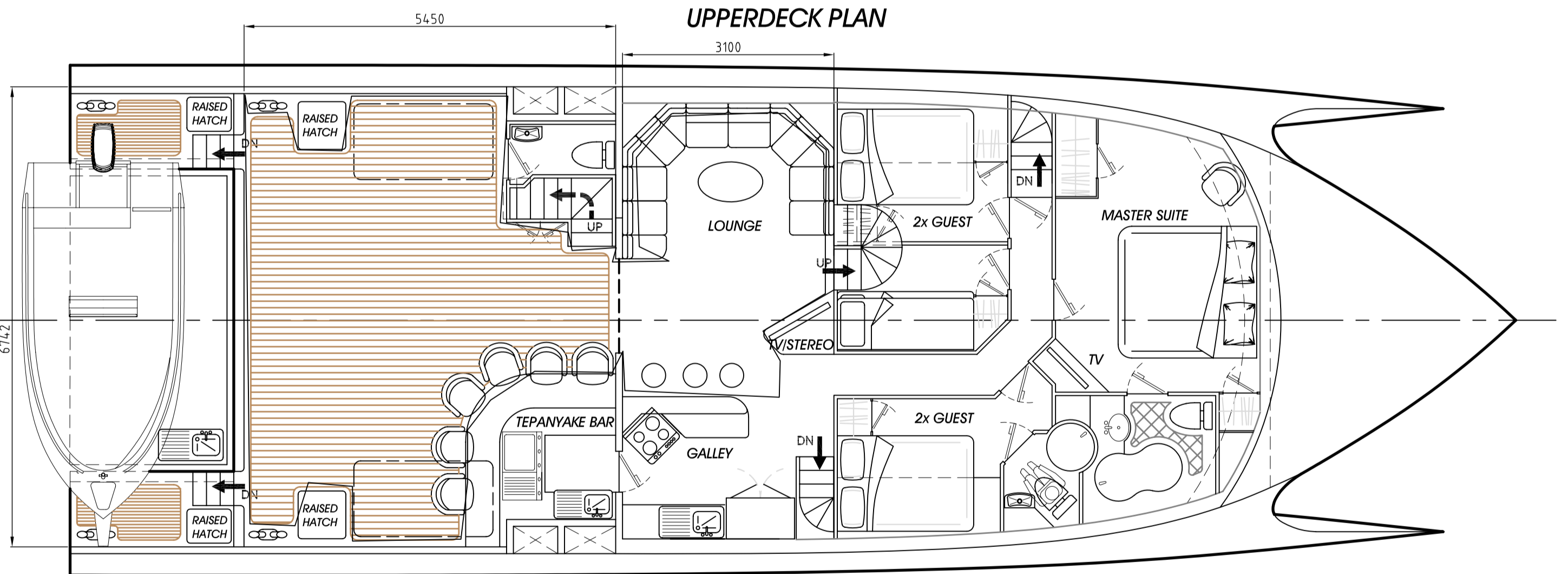
MAINDECK PLAN
